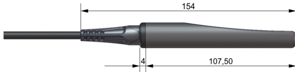
Figure 1: Dimensions (mm).
